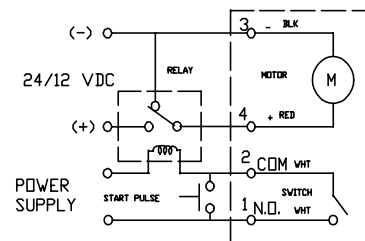
DRIVING CIRCUIT (REF.)
