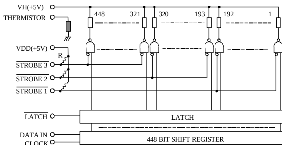
Fig. 3 Schematic Diagram
