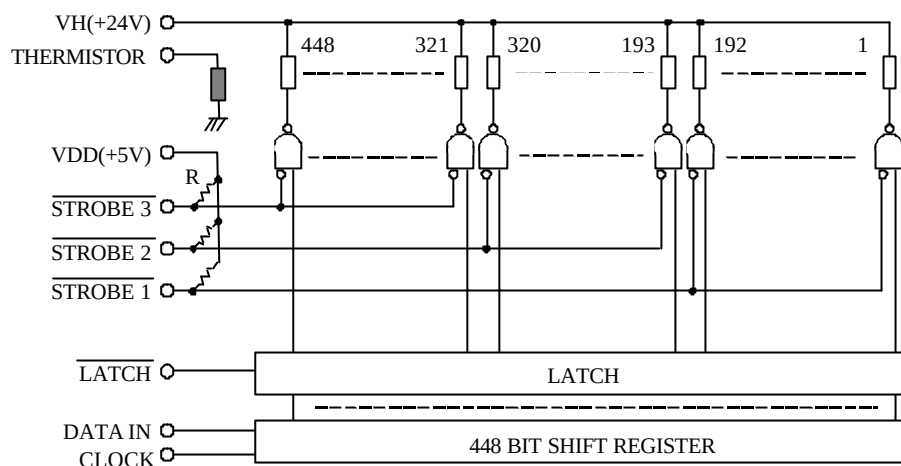
Fig. 3 Schematic Diagram
