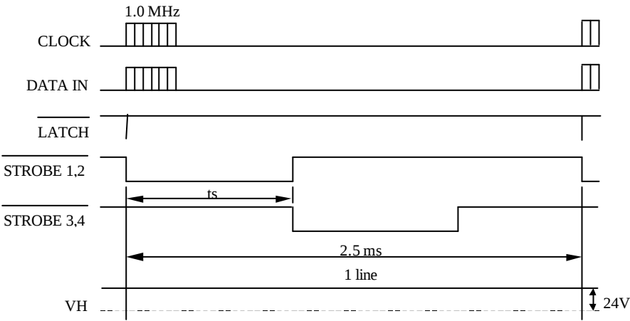
Fig. 2 Thermal Print Head (B72) Timing Chart
