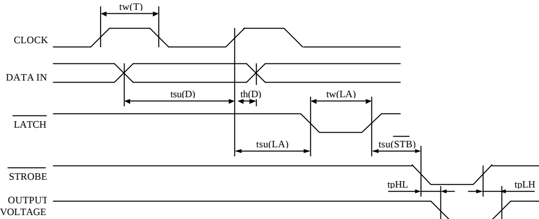
Fig. 2 Thermal Print Head (C56) Timing Chart
