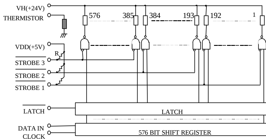
Fig. 3 Schematic Diagram
