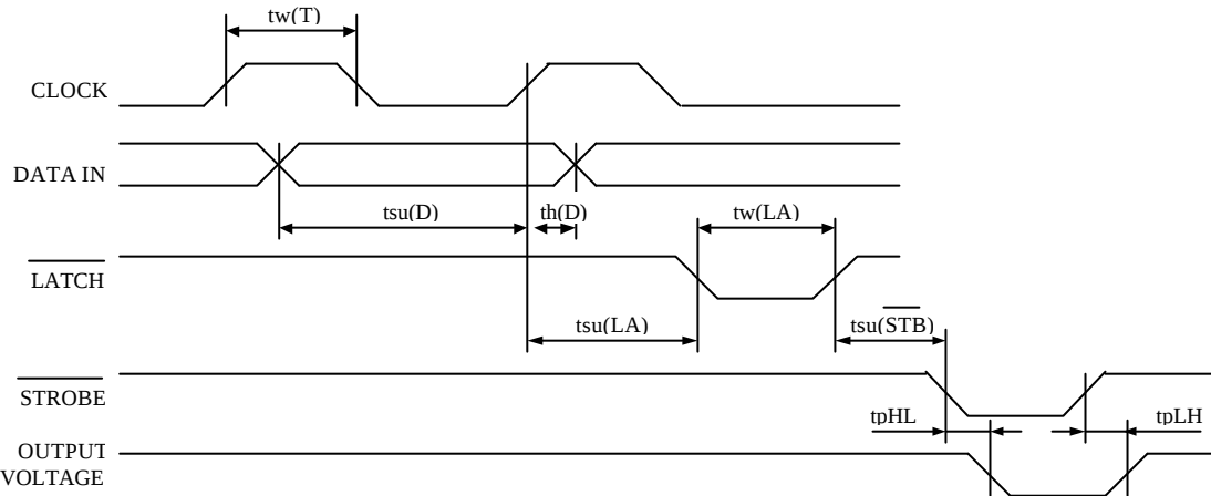
Fig. 2 Thermal Print Head (C128) Timing Chart
