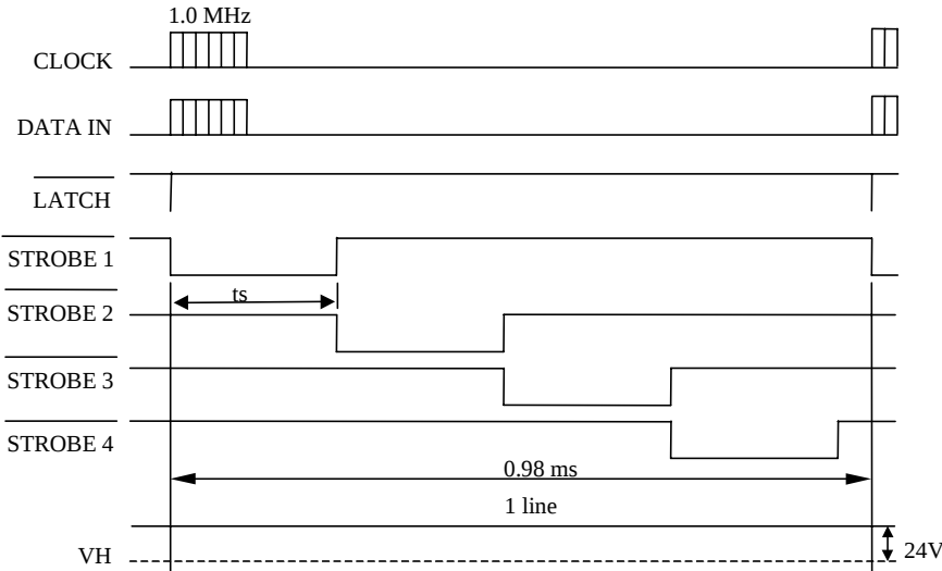
Fig. 2 Thermal Print Head (C216) Timing Chart
