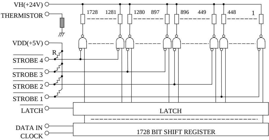
Fig. 3 Schematic Diagram
