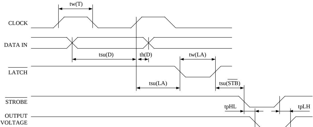
Fig. 2 Thermal Print Head (C216) Timing Chart
