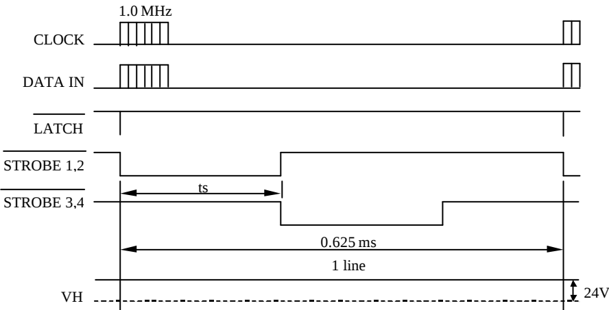
Fig. 2 Thermal Print Head (G80) Timing Chart
