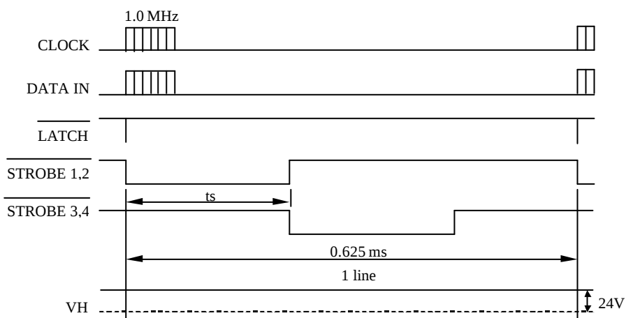
Fig. 2 Thermal Print Head (G104) Timing Chart
