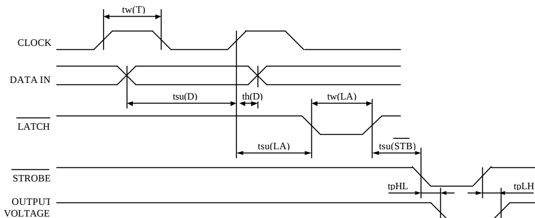
Fig. 2 Thermal Print Head (G104) Timing Chart
