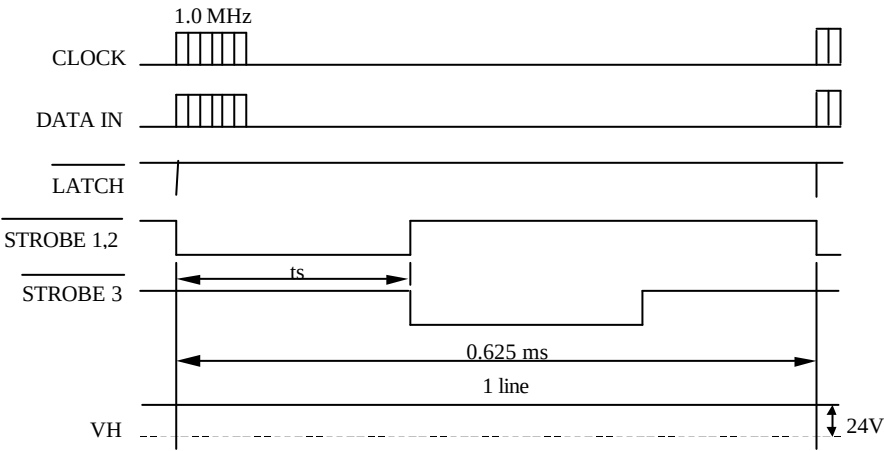
Fig. 2 Thermal Print Head (G56) Timing Chart
