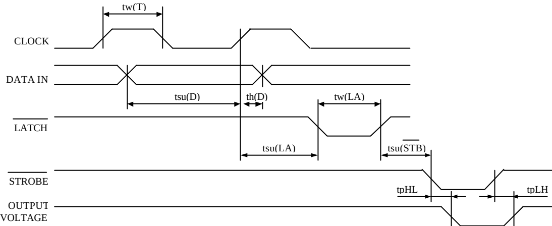
Fig. 2 Thermal Print Head (G56) Timing Chart
