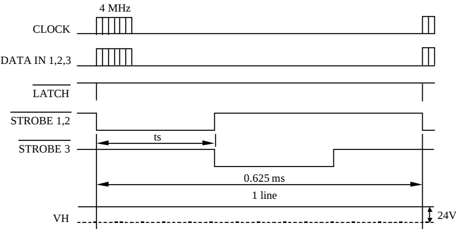
Fig. 2 Thermal Print Head (G80-3I) Timing Chart
