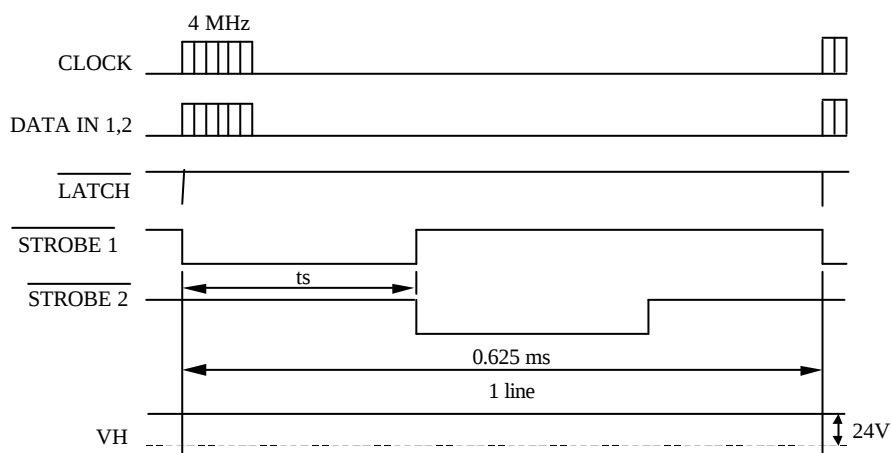
Fig. 2 Thermal Print Head (G56-2I) Timing Chart
