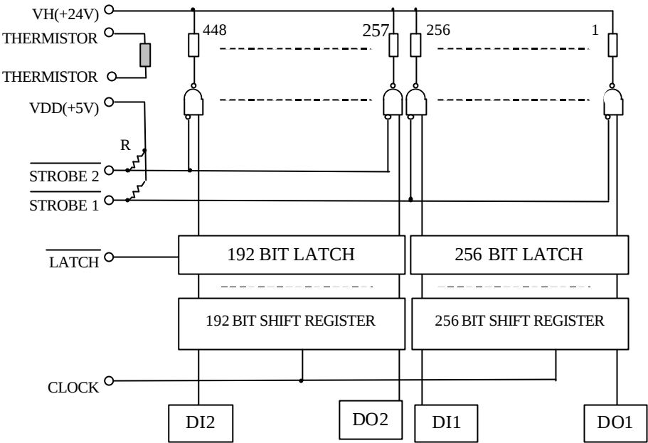
Fig. 3 Schematic Diagram
