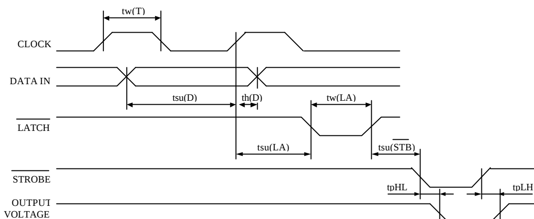
Fig. 2 Thermal Print Head (G56-2I) Timing Chart
