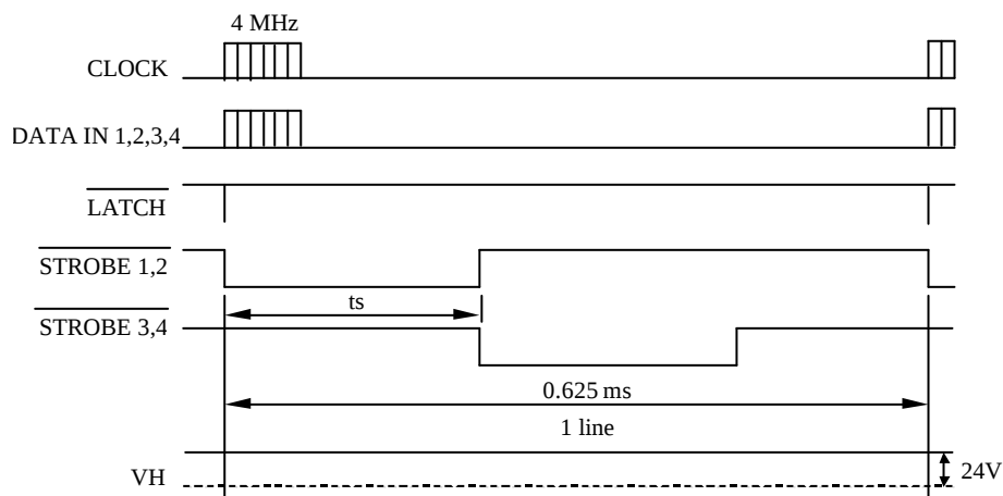
Fig. 2 Thermal Print Head (G104-4I) Timing Chart
