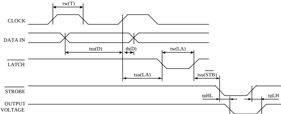
Fig. 2 Thermal Print Head (HA216-UH) Timing Chart
