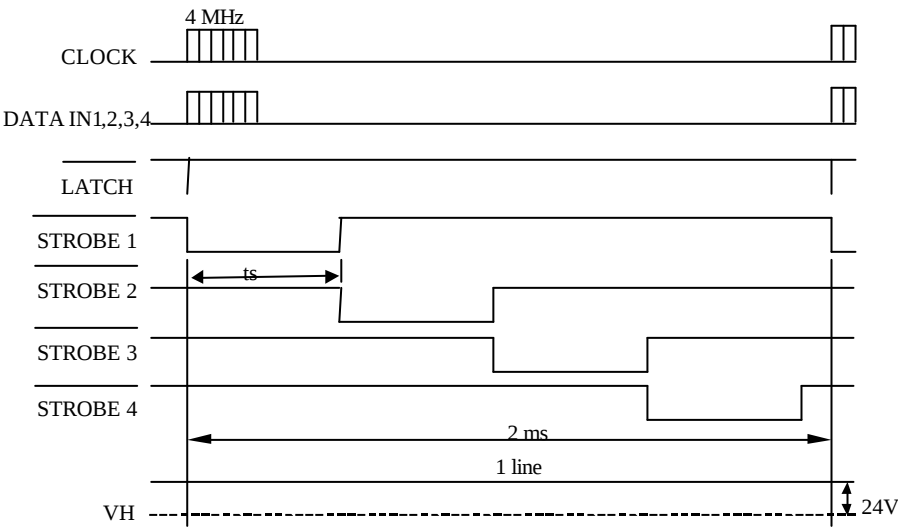
Fig. 2 Thermal Print Head (3G216-4I) Timing Chart
