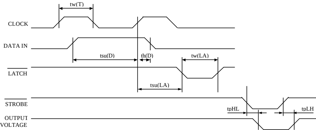
Fig. 2 Thermal Print Head (3G54-2I) Timing Chart
