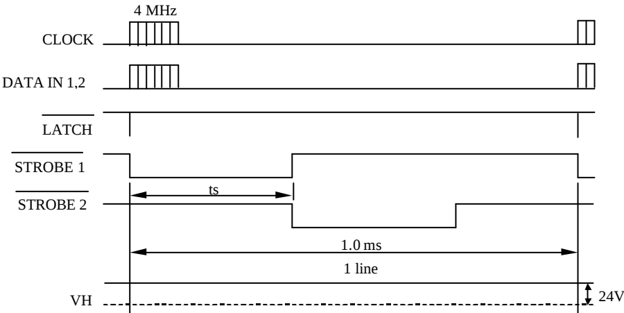
Fig. 2 Thermal Print Head (3G54-2I) Timing Chart
