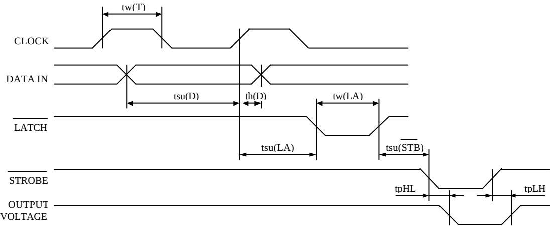
Fig. 2 Thermal Print Head (E48-PU) Timing Chart
