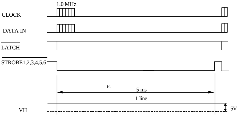
Fig. 2 Thermal Print Head (E48-PU) Timing Chart
