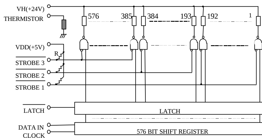
Fig. 3 Schematic Diagram
