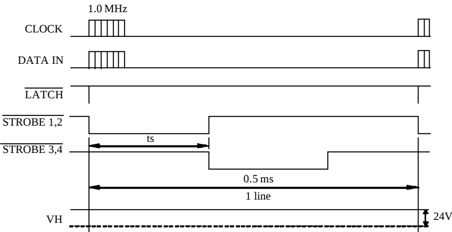
Fig. 2 Thermal Print Head (T104) Timing Chart
